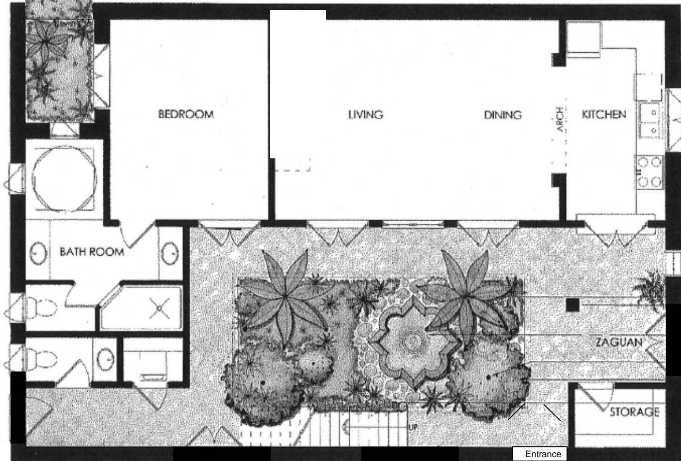
Main Floor
